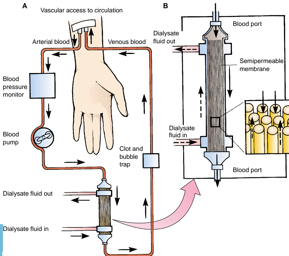
FIGURE 44-4 Hemodialysis system. (A) Blood from an artery is pumped into (B) a dialyzer where it flows through the cellophane tubes, which act as the semipermeable membrane (inset). The dialysate, which has the same chemical composition as the blood except for urea and waste products, flows in around the tubules. The waste products in the blood diffuse through the semipermeable membrane into the dialysate.
